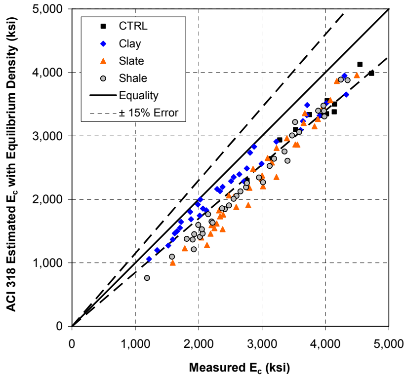
Figure 5-7: Measured modulus of elasticity compared to ACI 318 predicted with equilibrium density
